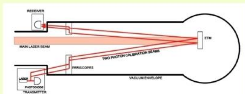
Figure 19 Schematic of the photon calibration system.
