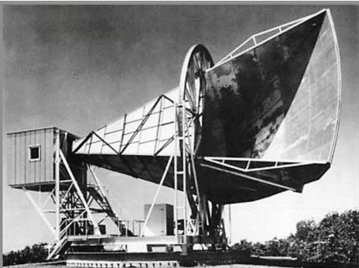
↑: Penzias-Wilson "sugarscoop" antenna, aperture \sim 20 ft \times 20 ft; ↓: Herouni reflector antenna, aperture 177 ft dia
