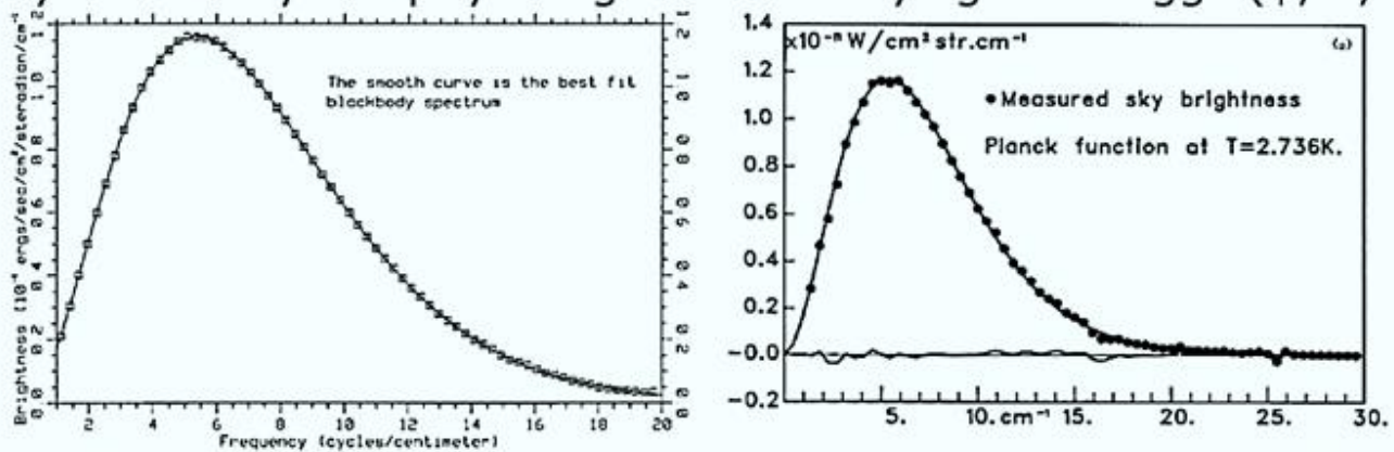
The published energy spectra of the cosmic microwave background, as measured by COBE (left) and COBRA. Credit: J. C. Mather et al., 1990 (left); H. P. Gush et al., 1990
