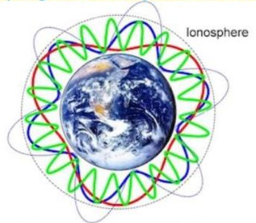
Electromagnetic waves created by lightning flashes and trapped between the ground and the ionosphere - here shown in blue, green, and red - circle around Earth, creating Schumann resonance. (Image Credit: NASA/Simoes)
