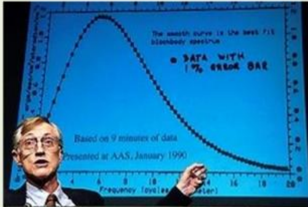
OFFICIAL 2006 NASA PHOTO SHOWING JOHN MATHER DISCOVERY OF THE BLACKBODY FORM OF THE COSMIC MICROWAVE BACKGROUND RADIATION WITH THE NASA COBE SATELLITE; THE MATHER FRAUDULENT EXPERIMENT
