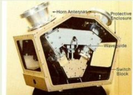
OFFICIAL 2006 LAWRENCE BERKELEY LAB PHOTO SHOWING GEORGE SMOOT DISCOVERY OF THE ANISOTROPY MAP OF COSMIC MICROWAVE BACKGROUND RADIATION ; SMOOT EXPERIMENT
