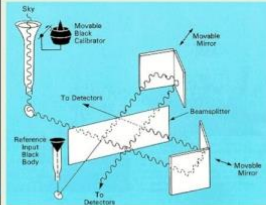
OFFICIAL 2006 NASA PHOTO SHOWING JOHN MATHER DISCOVERY OF THE BLACKBODY FORM OF THE COSMIC MICROWAVE BACKGROUND RADIATION WITH THE NASA COBE SATELLITE; THE MATHER FRAUDULENT EXPERIMENT
