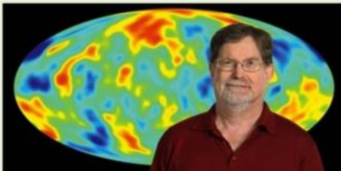
OFFICIAL 2006 LAWRENCE BERKELEY LAB PHOTO SHOWING GEORGE SMOOT DISCOVERY OF THE ANISOTROPY MAP OF COSMIC MICROWAVE BACKGROUND RADIATION ; SMOOT EXPERIMENT
