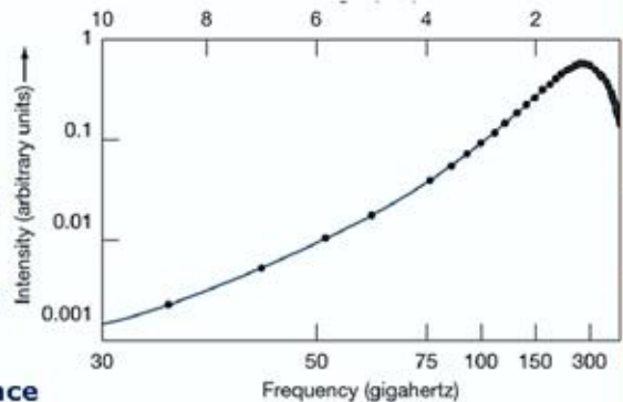
Nobel Prize duly followed in 1978. COSMIC BLACKBODY SPECTRUM
